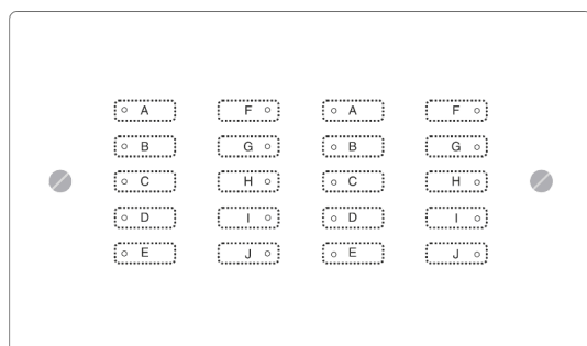
Example: WVF-10010-XX (Double keypad alignment)
